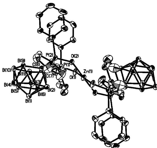
Figure 2. The crystal structure of complex 2 . The H atoms were omitted for clarity.
