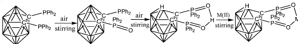
Scheme 1. The rational reaction process for the preparation of the complexes 1 to 3 [ M = \text{Cu}(\mathbf{1}) , \text{Zn}(\mathbf{2}) , \text{Ni}(\mathbf{3}) ].
