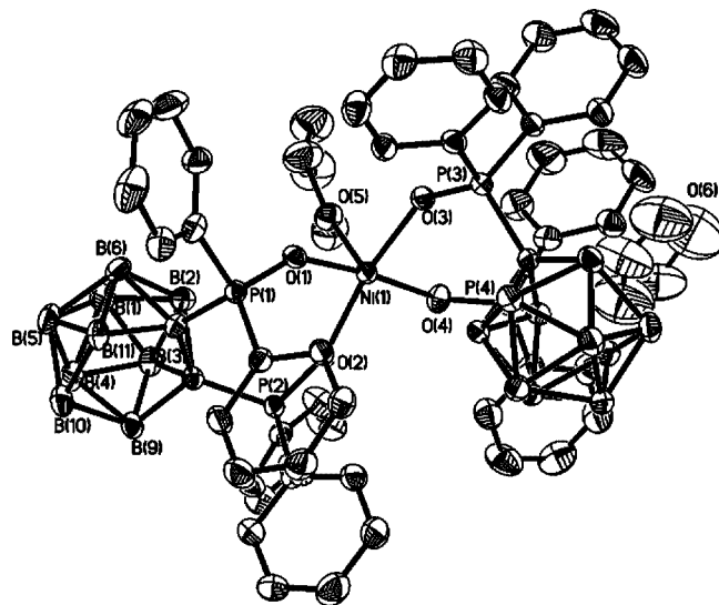
Figure 3. The crystal structure of complex 3 . The H atoms were omitted for clarity.
