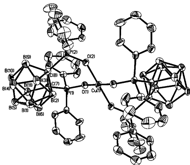
Figure 1. The crystal structure of complex 1 . The H atoms were omitted for clarity.
