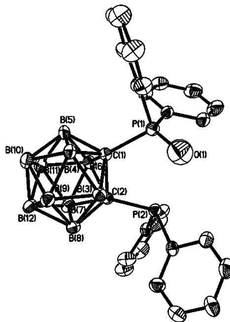
Figure 4. The crystal structure of compound 4 . The H atoms were omitted for clarity.
