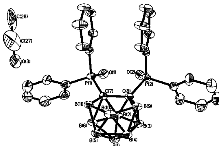
Figure 5. The crystal structure of compound 5 . The H atoms were omitted for clarity.
