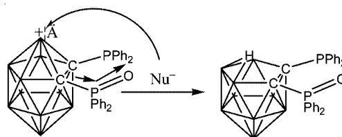
Scheme 2. Proposed mechanism for the partial degradation of compound 4 .
